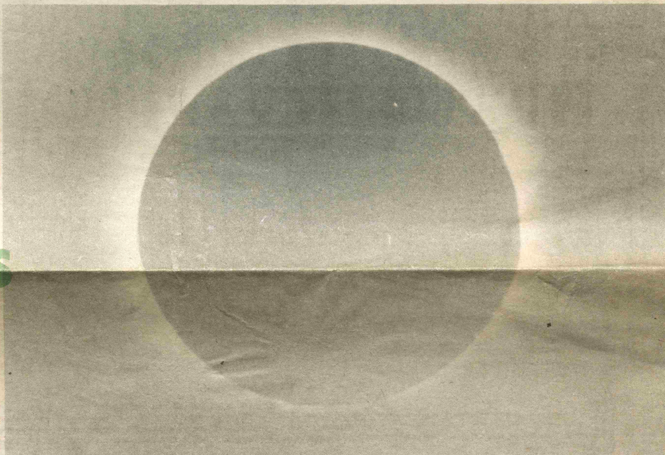
The solar corona taken by George Ball at the solar eclipse of February 26, 1979. Mr. Ball is a member of the Victoria Centre of the Royal Astronomical Society of Canada
