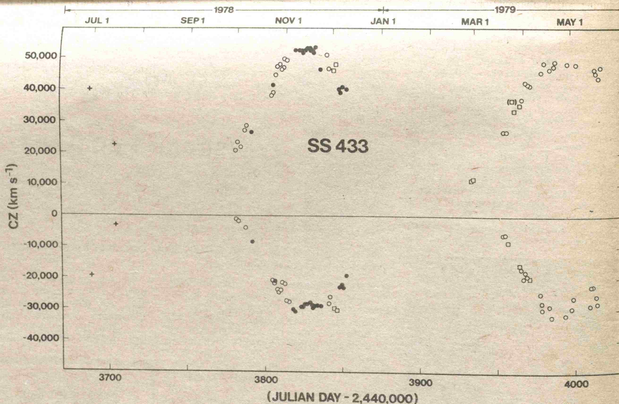
The fingerprint of SS 433
